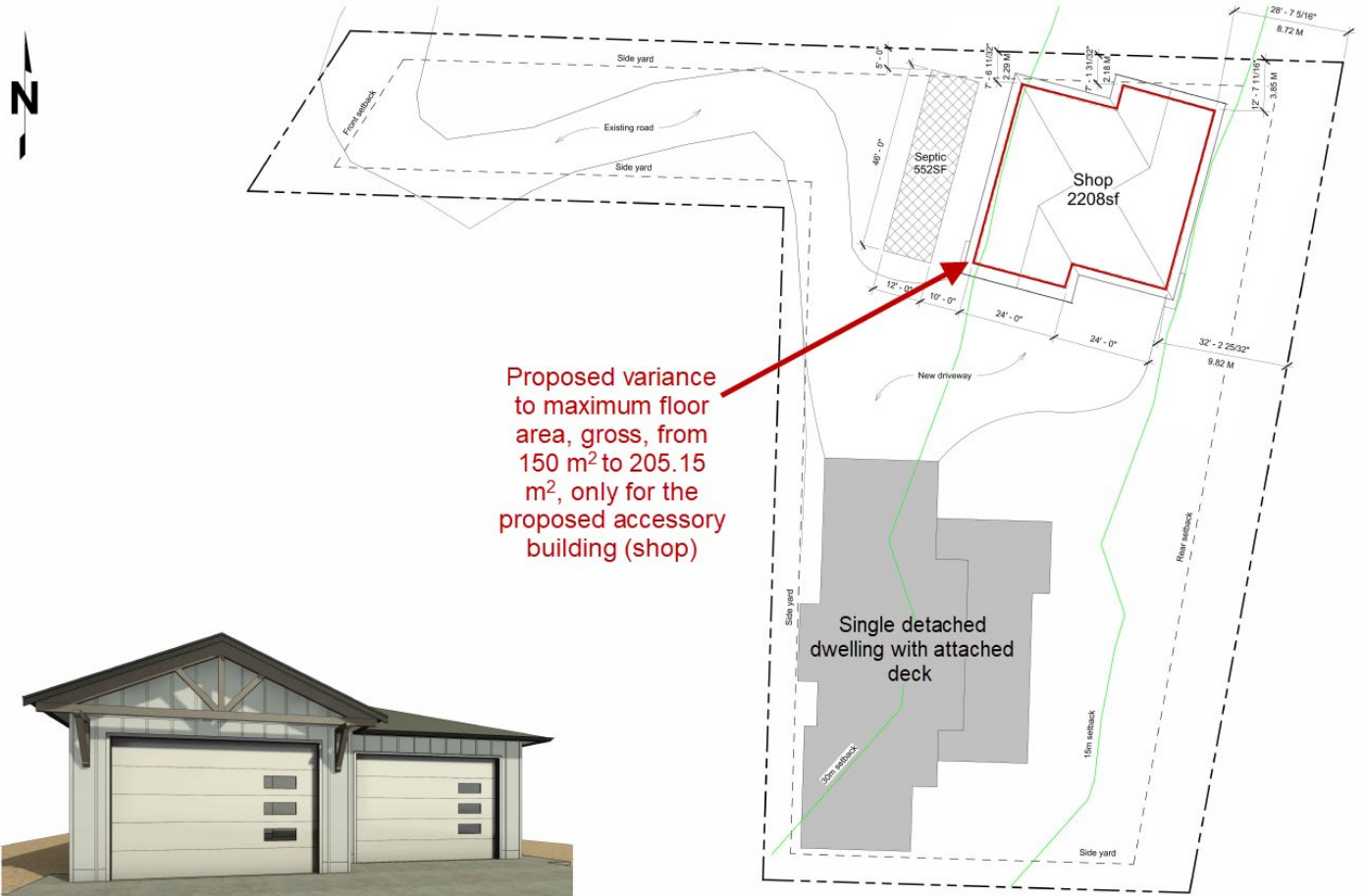
1 Site Plan 1/16" = 1'-0"
