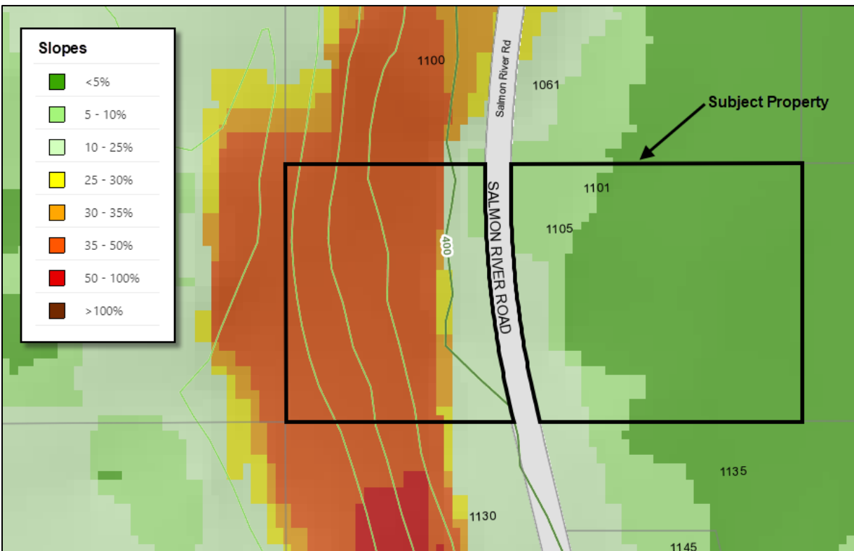
Slopes
